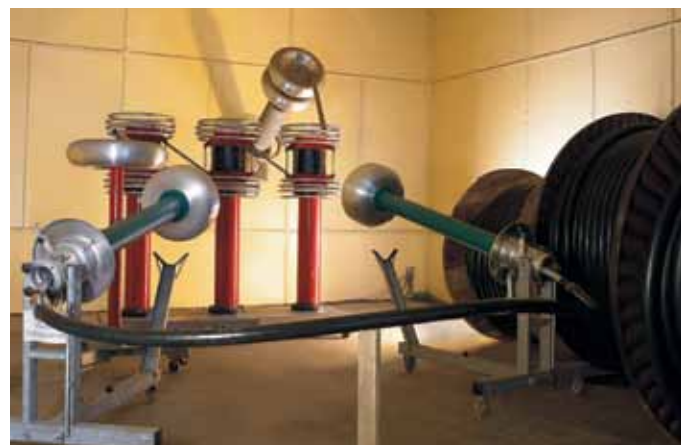
Figure 3 : ULTRA MODERN HV TESTING LAB
